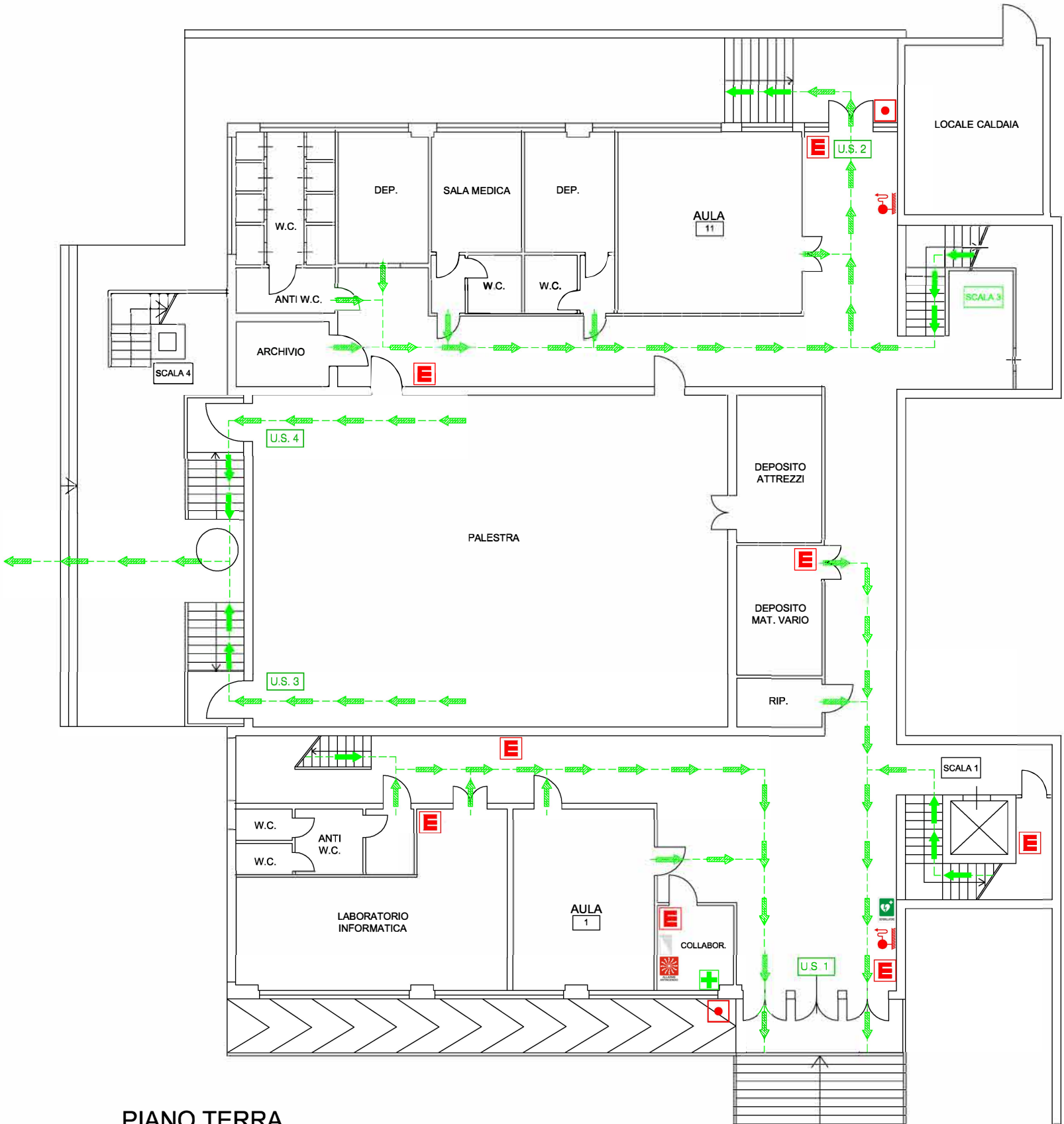
PIANO TERRA
